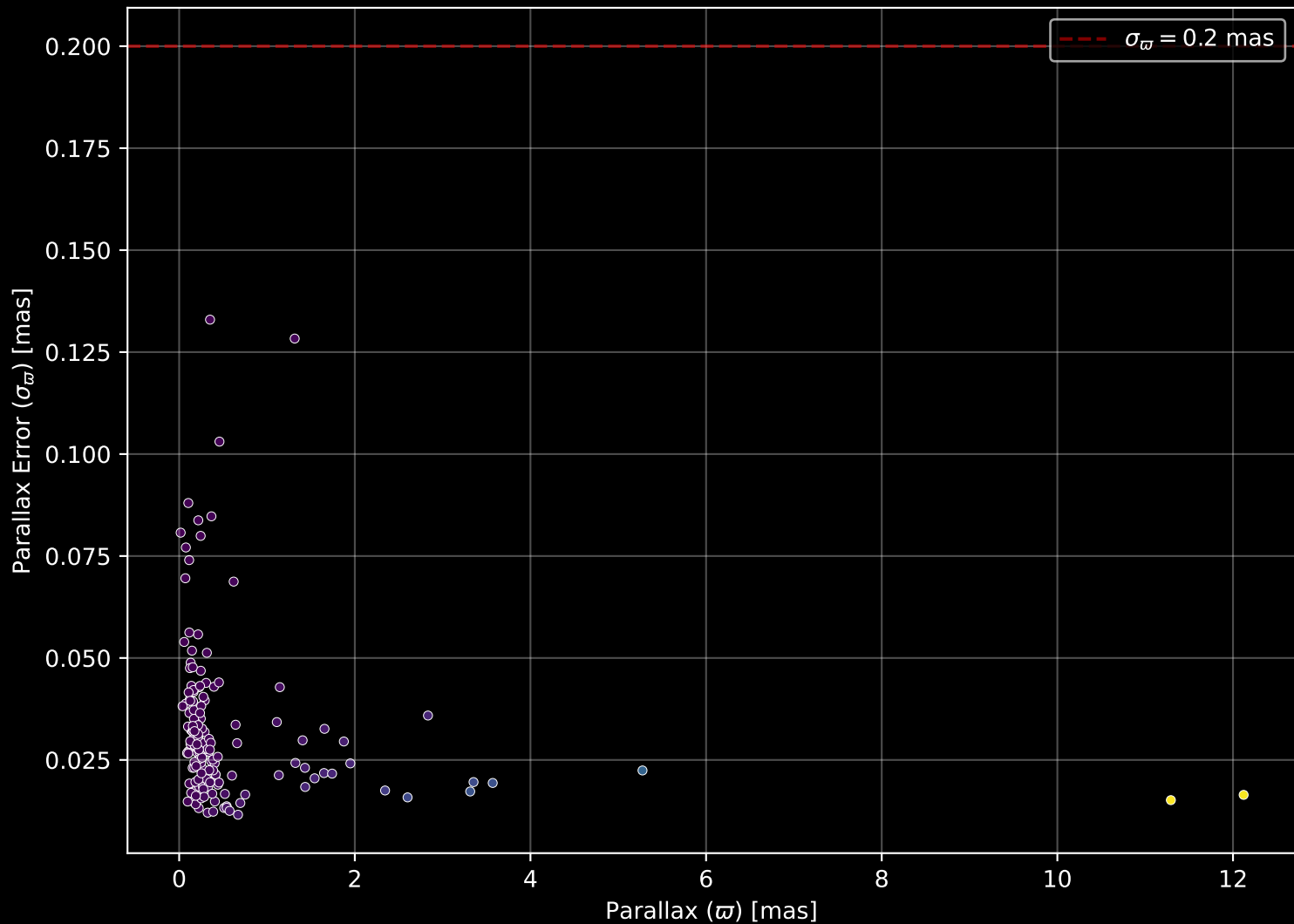
APOGEE DR17 Field: [068-04] Parallax Quality (n= 168)
