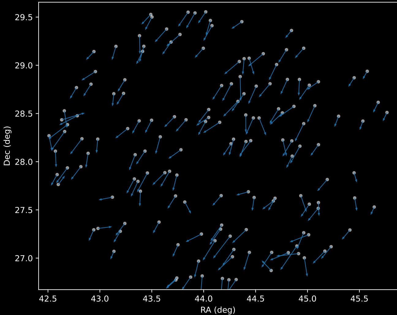
APOGEE DR17 Cluster 0 Proper Motion Vectors (n=150)
